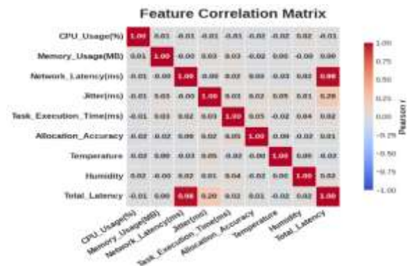
Fig. 4. Correlation Matrix of features
